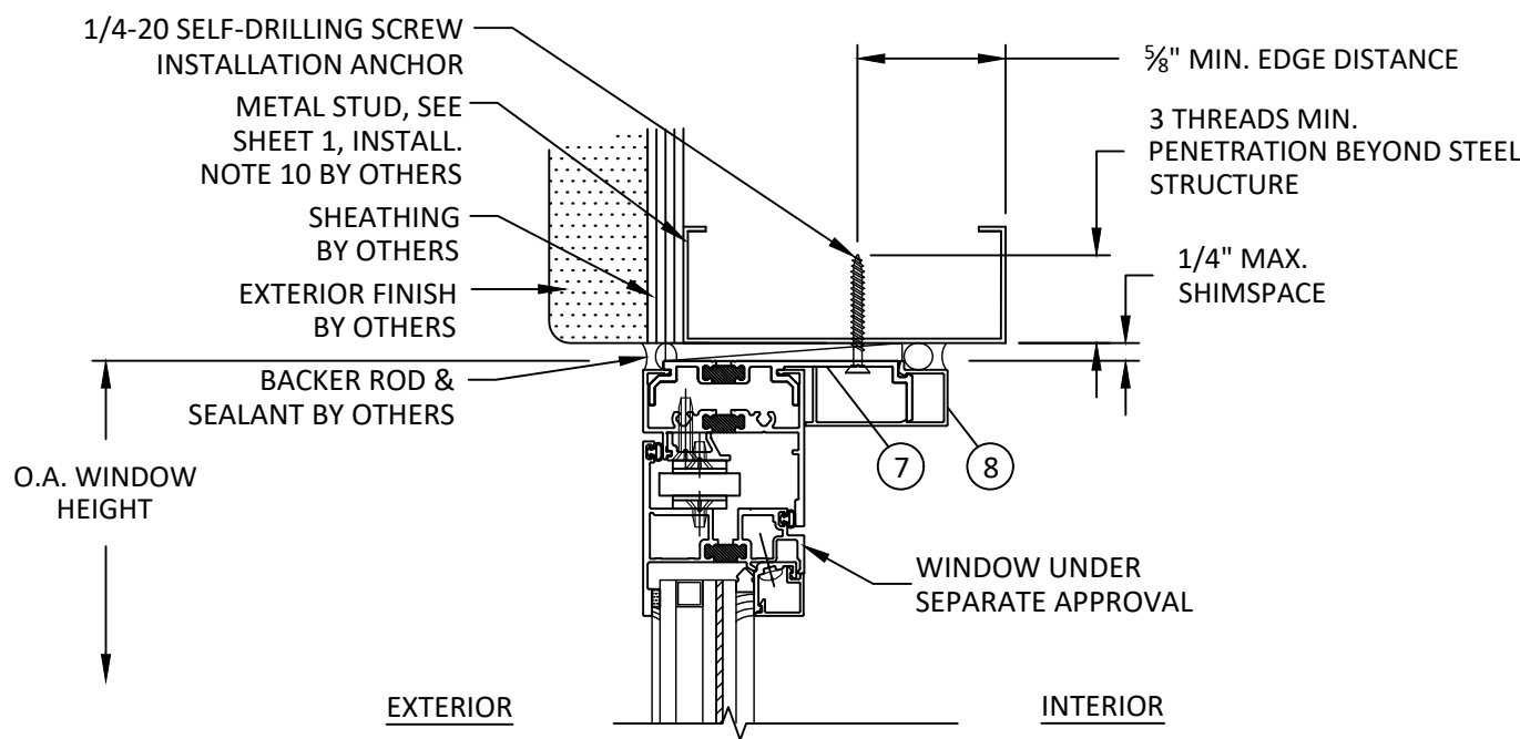
G 3 VERTICAL SECTION HEAD - METAL STUD UNCLIPPED MULLION (ALT. ANCHOR STRAP)
