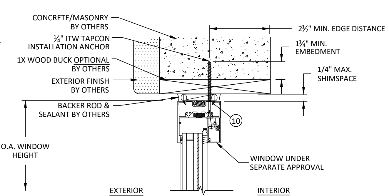
I 3 VERTICAL SECTION HEAD - 1X WOOD BUCK UNCLIPPED MULLION
