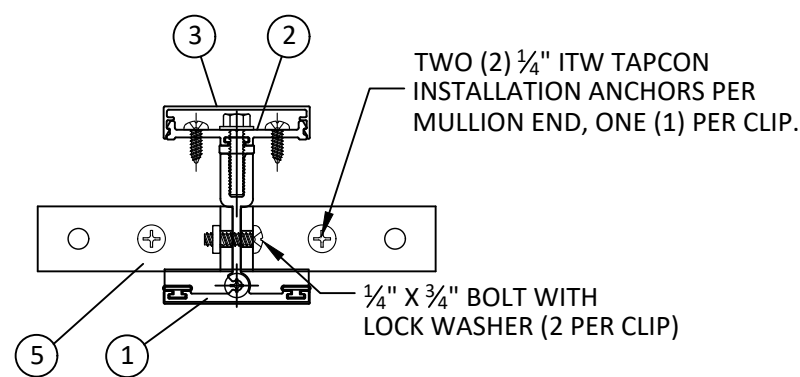
D 2 HORIZONTAL SECTION CONCRETE/MASONRY MULLION CLIP
