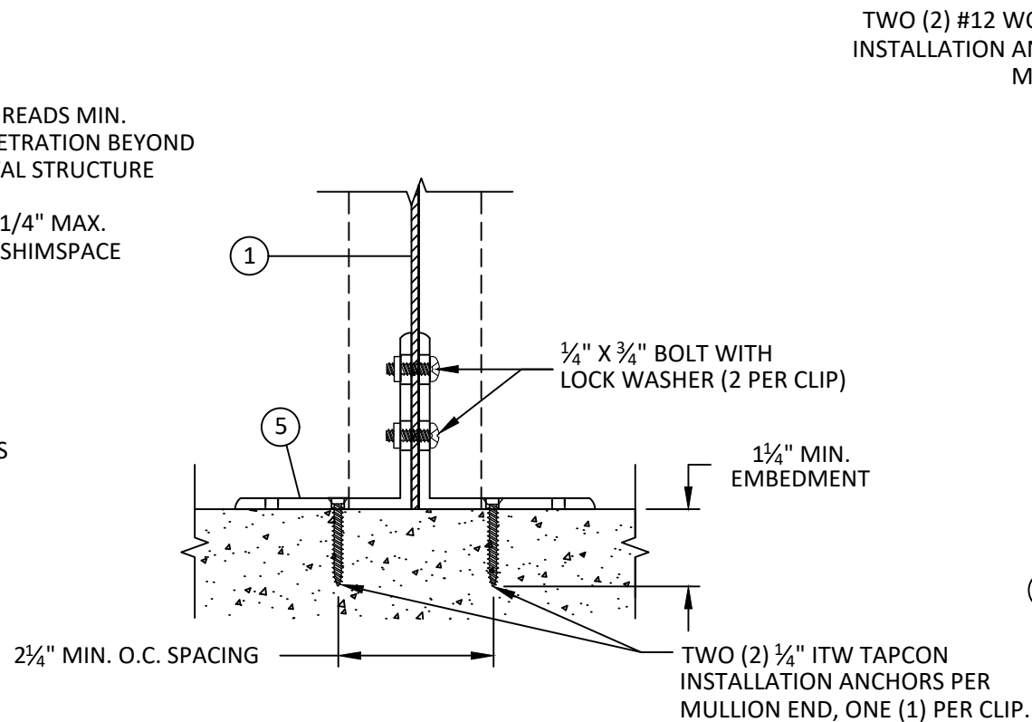
C 2 FRONT VIEW SILL - CONCRETE/MASONRY MULLION CLIP
