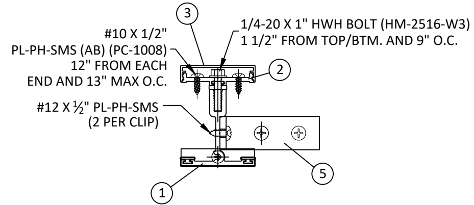
F 2 HORIZONTAL SECTION 2X WOOD MULLION CLIP
