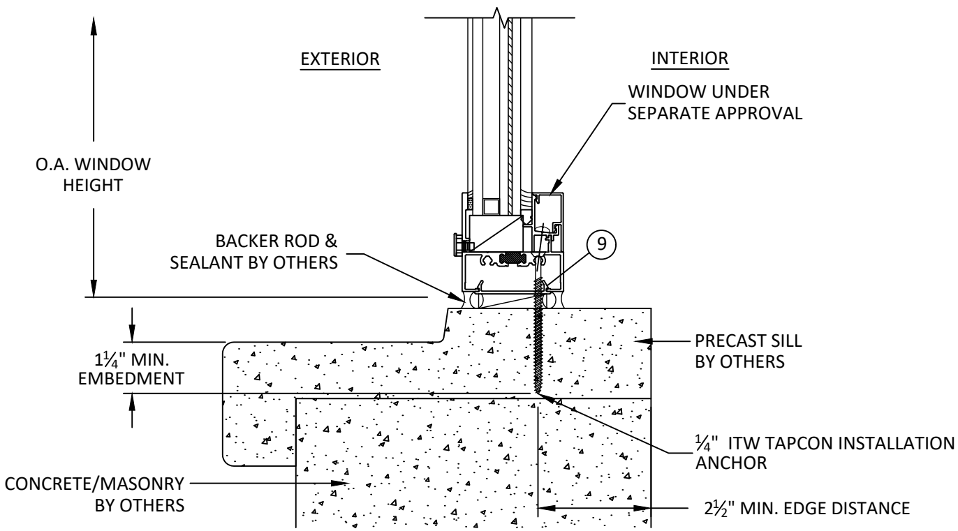
J 3 VERTICAL SECTION SILL - PRECAST SILL UNCLIPPED MULLION
